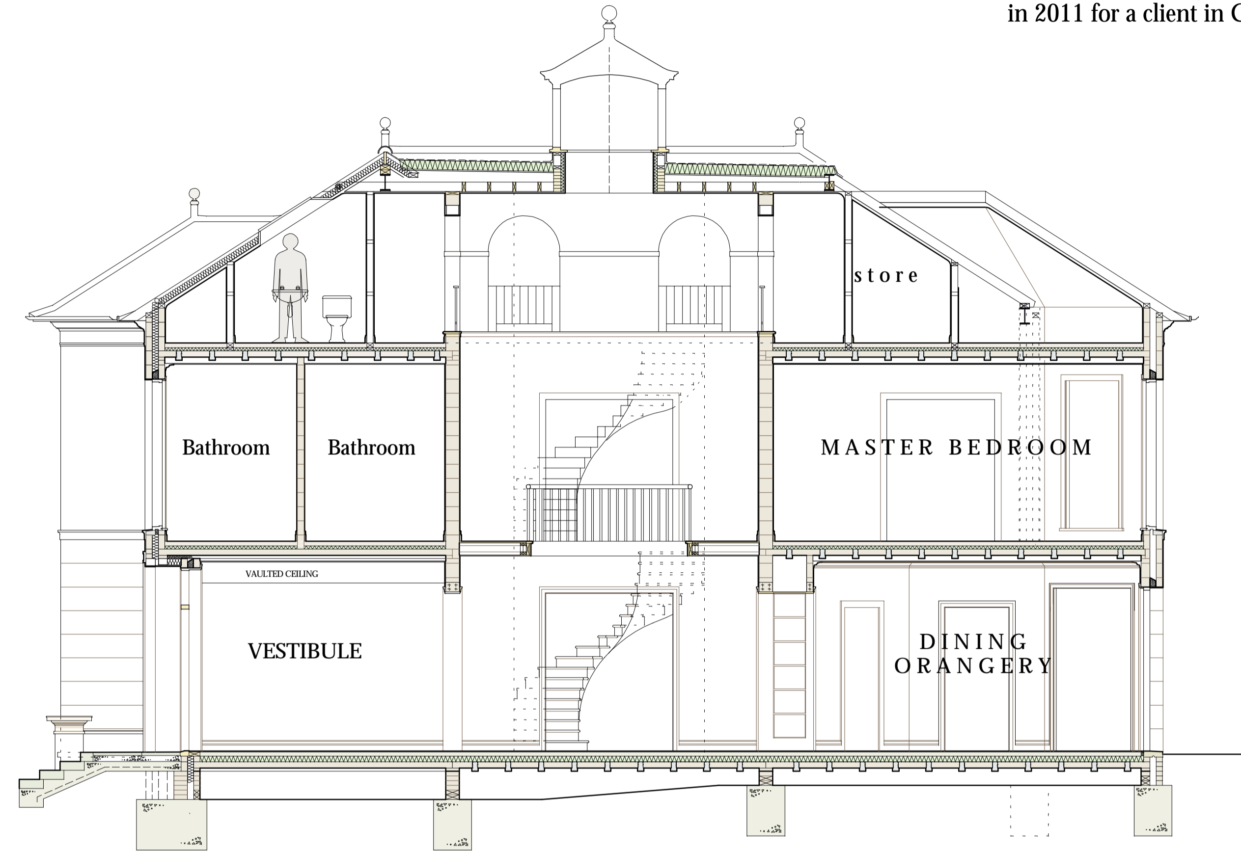
SECTION
